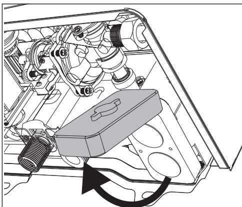
fig. 18 - Opening the battery box
