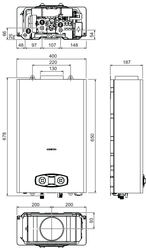
fig. 21 - Dimensions and connections ZEFIRO ECO 14
