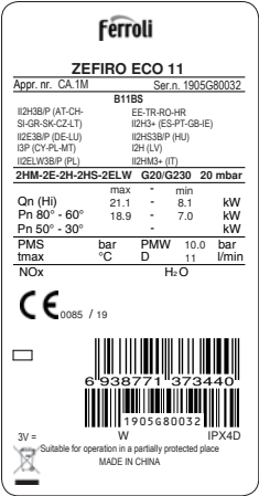
fig. 7 - Rating label
