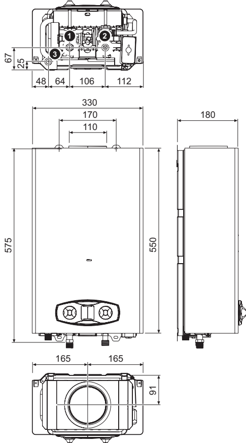
fig. 20 - Dimensions and connections ZEFIRO ECO 11
