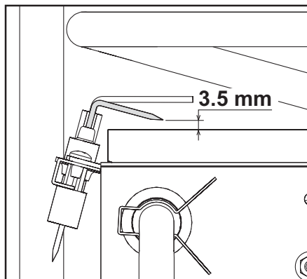
fig. 16 - Electrode position
