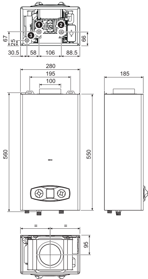
fig. 19 - Dimensions and connections ZEFIRO ECO 6
