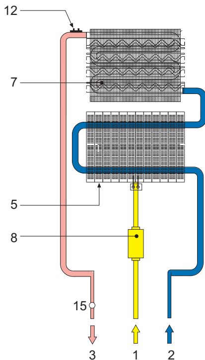
fig. 25 - Hydraulic circuit
