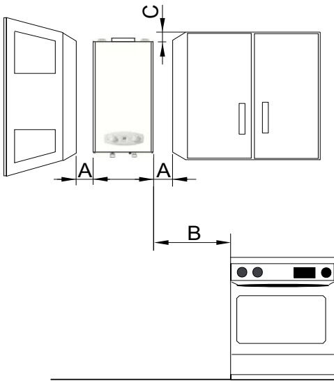
fig. 5 - Minimum distances
