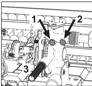
fig. 9 - Water flow adjustment screws
